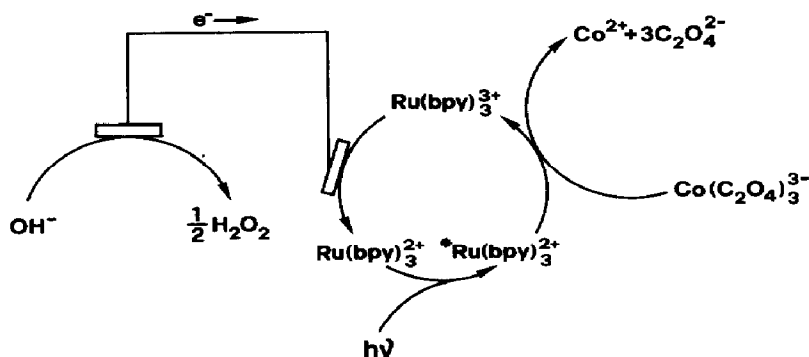
Fig. 27. An example of the use of \text{Ru(bpy)}_3^{2+} as LAS: light is used to generate electrical energy and to carry on a net redox process [201].
