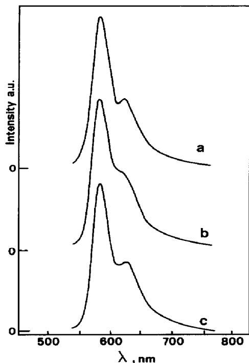
Fig. 44. Emission spectra in nitrile solution at 84 K of \text{Ru}(\text{bpy})_3^{2+} (a), \text{Ru}(\text{bpy})_2(\text{i-biq})^{2+} (b), and \text{Ru}(\text{bpy})(\text{i-biq})^{2+} (c) [131].
