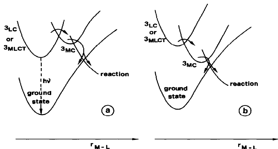
Fig. 14. Schematic representation of two limiting cases for the relative positions of ^3MC and ^3LC (or ^3MLCT ) excited states.
