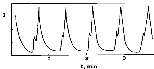
Fig. 32. Oscillating chemiluminescence observed using \text{Ru(bpy)}_3^{2+} as LES in the Belousov–Zhabotinskii reaction [202] (see text).
