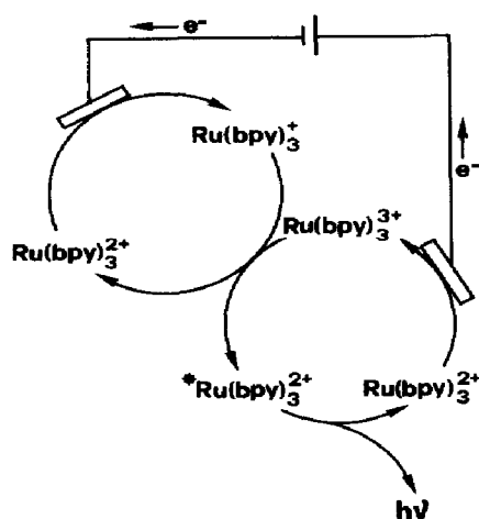
Fig. 31. An example of the use of \text{Ru(bpy)}_3^{2+} as LES: electrical energy is converted into light energy [59].
