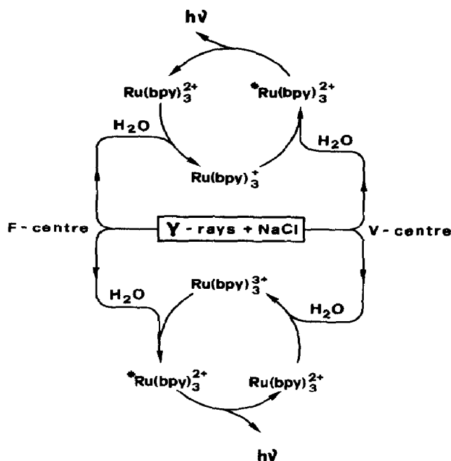
Fig. 33. An example of the use of \text{Ru}(\text{bpy})_3^{2+} as LES: chemical energy stored into \gamma -irradiated solids is converted into light (sensitized luminescence) [203].
