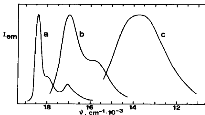
Fig. 34. Emission spectra of \text{Ru}(\text{i-biq})_3^{2+} (a), \text{Ru}(\text{i-biq})_2(\text{bpy})^{2+} (b), and \text{Ru}(\text{i-biq})_2\text{Cl}_2 (c) [217].
