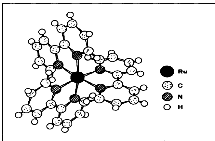
Fig. 13. Structure of \text{Ru}(\text{bpy})_3^{2+} [52].
