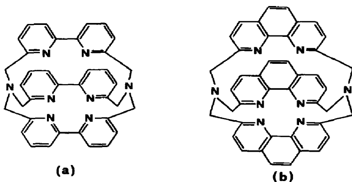
Fig. 22. Cage-type polypyridine ligands [147].
