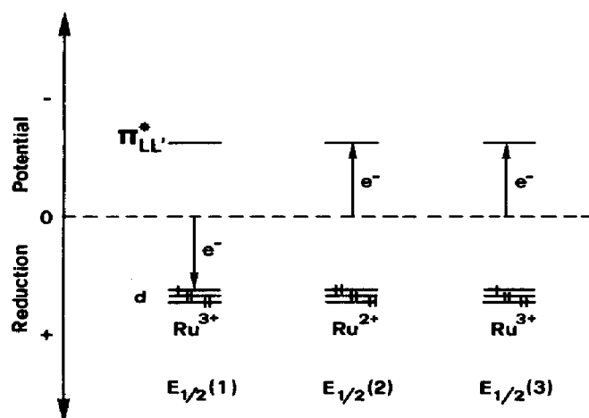
Fig. 37. Schematic diagram showing pictorially the three reduction processes relevant to a discussion of the correlation between spectroscopic and electrochemical properties in a \text{Ru}(\text{LL}')_2 unit.
