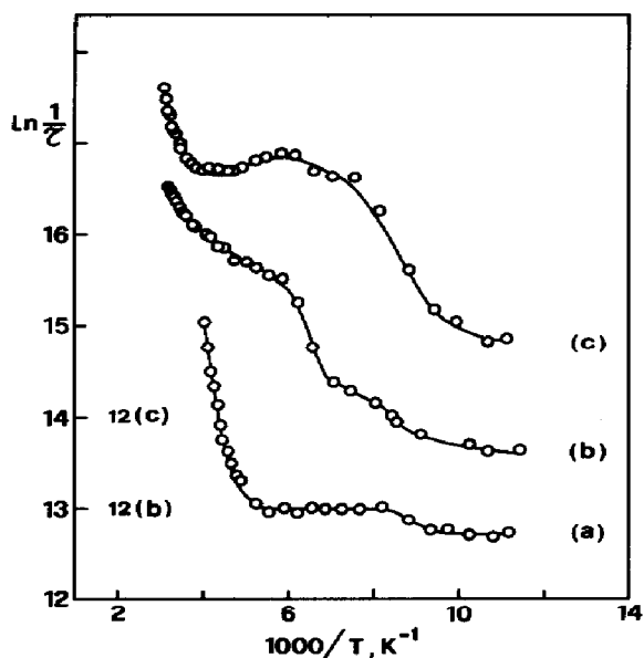
Fig. 35. Temperature dependence of the emission lifetime of \text{Ru}(\text{biq})_3^{2+} (a), \text{Ru}(\text{bpy})_2(\text{CN})_2 (b), and \text{Ru}(\text{tapen})_3^{2+} (c). Curves (b) and (c) are shifted along the ordinate axis as indicated.
