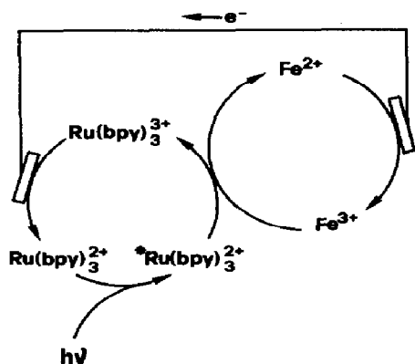
Fig. 26. An example of the use of \text{Ru(bpy)}_3^{2+} as LAS: light energy is converted into electrical energy (photogalvanic effect) [199].
