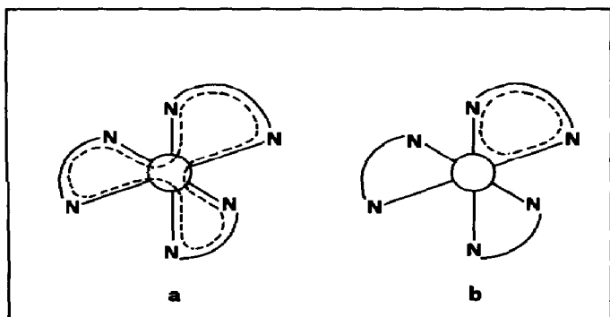
Fig. 15. Pictorial description of the electron promoted to the \pi_L^* orbital: (a) multichelate ring delocalized orbital; (b) single chelate ring localized orbital [65].
